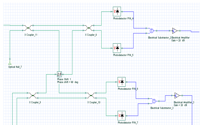
Figure 4: Coherent Detection of Optical OFDM
