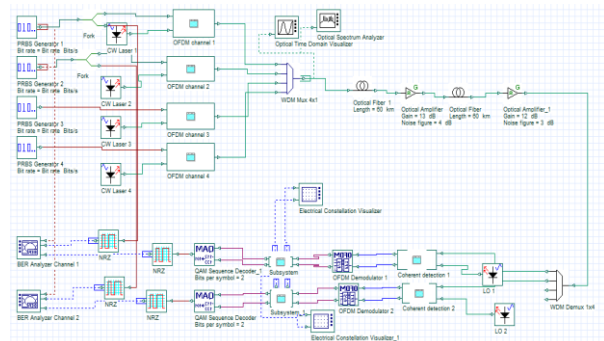
Figure 5: Coherent WDM Optical OFDM system
