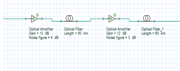
Figure 3: Optical Transmission Link.
