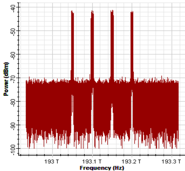
Figure 8: (b) Optical signal in the Fiber
