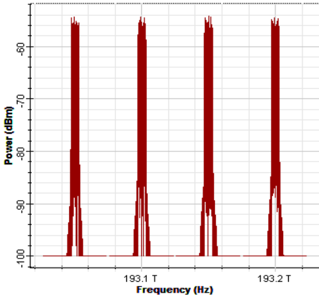
Figure 8: (a) Signal after WDM MUX.
