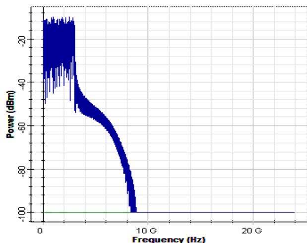
Figure 7: Modulated OFDM Signal in Frequency Domain for each OFDM Channel.
