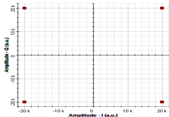
Figure6: 4 QAM Encoder Constellation Diagram
