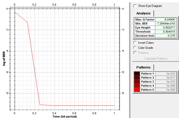
Figure 10: Minimum BER with Optical filter
