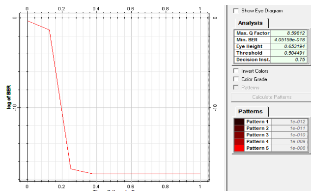
Figure 9: Minimum BER with Phase Modulator
