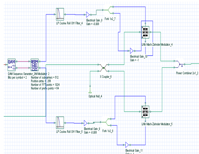
Figure 2: Optical OFDM Transmitter
