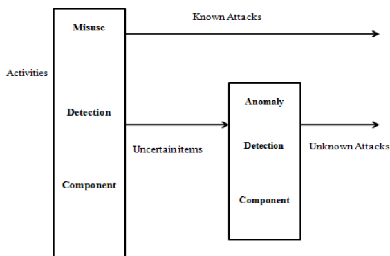
Figure 2: Hybrid classifier
