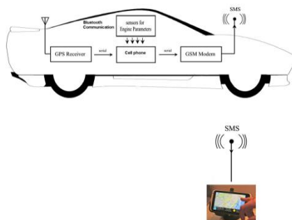
Figure 2: The system architecture: GPS tracking and GSM modules.
