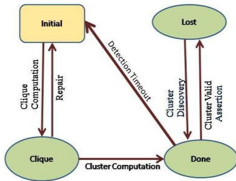
Finite State Machine of the Cluster Formation Protocol
