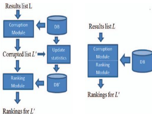
Fig 3: Approximation algorithm.
