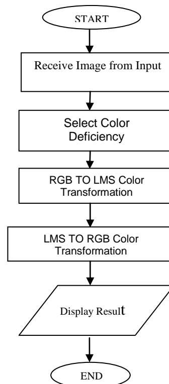
Fig 4.Algorithm for Simulation of Image
