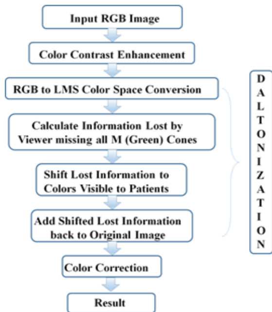
Fig 3.Process flow diagram of the proposed paper
