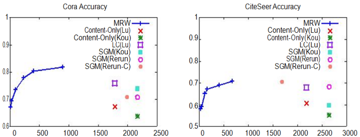
Fig. 5. Citation datasets results compared to supervised relational learning methods. The x-axis indicates number of labeled instances and y-axis indicates labeling accuracy.
