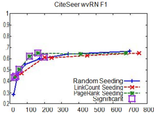
Fig. 3. wvRN results varying the seeding method. The x-axis indicates number of labeled instances and y-axis indicates labeling macro-averaged F1 score. Square block around a point indicates statistical significance with p < 0.05 .
