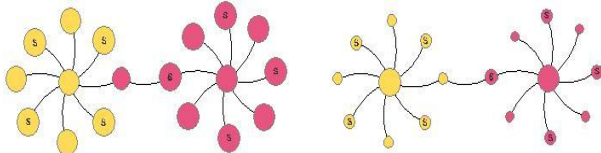
Fig. 8. Right: Labels predicted by wvRN. Left: Labels predicted by MRW. The seed nodes are labeled S and relative sizes of nodes in the graphs indicate how confident the algorithm is in its prediction and how strongly a node will influence its neighbors.
