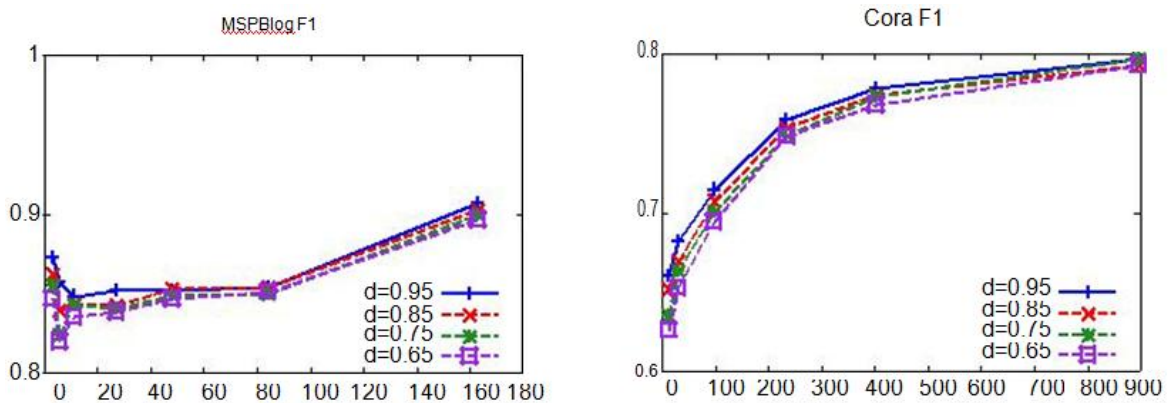
Fig. 7. Results on three datasets varying the damping factor. The x-axis indicates number of labeled instances and y-axis indicates labeling macro-averaged F1 score.
