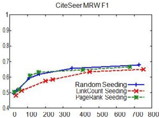
Fig. 4. MRW results varying the seeding method. The x-axis indicates number of labeled instances and y-axis indicates labeling macro-averaged F1 score. Square block around a point indicates statistical significance with p < 0.05 .
