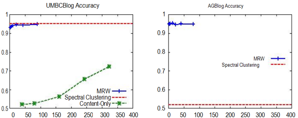
Fig. 6. Two political blog datasets results compared to spectral clustering methods. The x-axis indicates number of labeled instances and y-axis indicates labeling accuracy.
