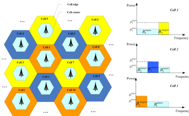
Fig. 2. Reference system layout and standard frequency planning for SFR
