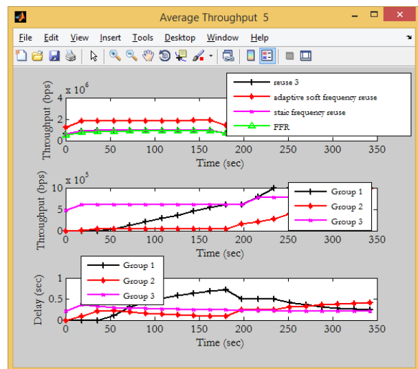
Fig 5(a) Average throughput of cell 5
