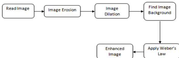
fig. 2.2.1 Block diagram of Background Detection by Erosion & Dilation
