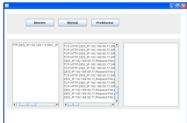
Figure 4. Classification output
