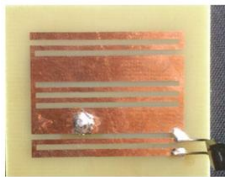
Fig:4 (a) Reconfigured antenna
