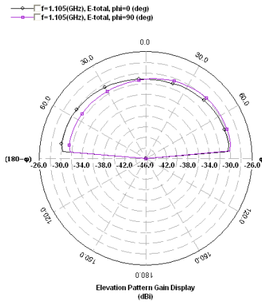
Fig:5(a) Radiation patterns of the antenna at 1.1 GHz
