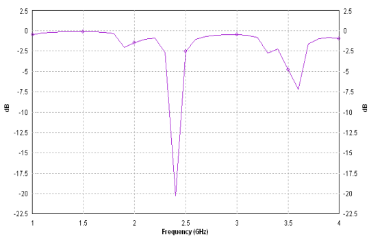
(b) Simulated return loss
