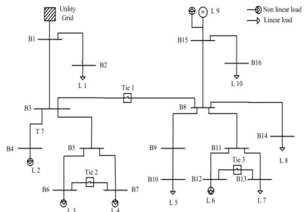
Fig.2. Single line diagram of the IEEE 16-bus test system
