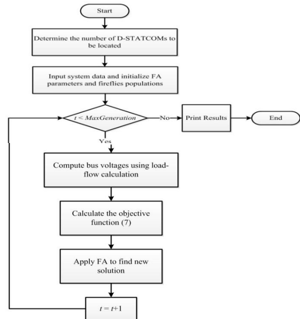
Fig1.FA implementation to solve the D-STATCOM placement and sizing problem
