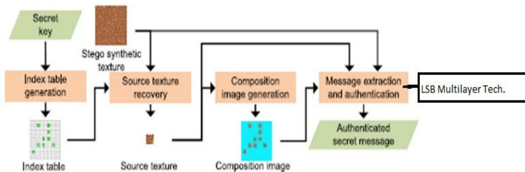
Fig. (b) Message Extracting Procedure
