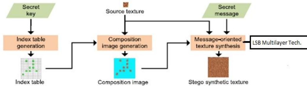
Fig. (a) Message Embedding Procedure
