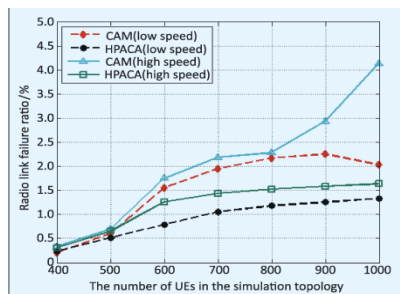
Fig. 2 The no. Of UEs in simulation topology vs Radio Link Failure ratio
