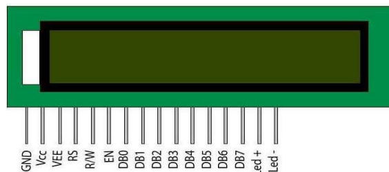
Fig. 5 The 16x2 LCD Display is used to provide information regarding the location.
