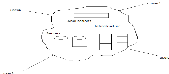
Fig. 1. Cloud Computing
