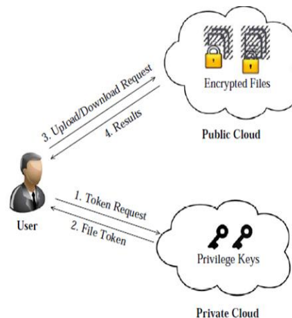
Fig. Architecture for Authorized Deduplication
