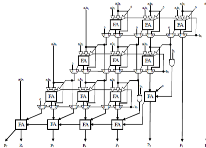
Fig 2. 4 × 4 row-bypassing multiplier
