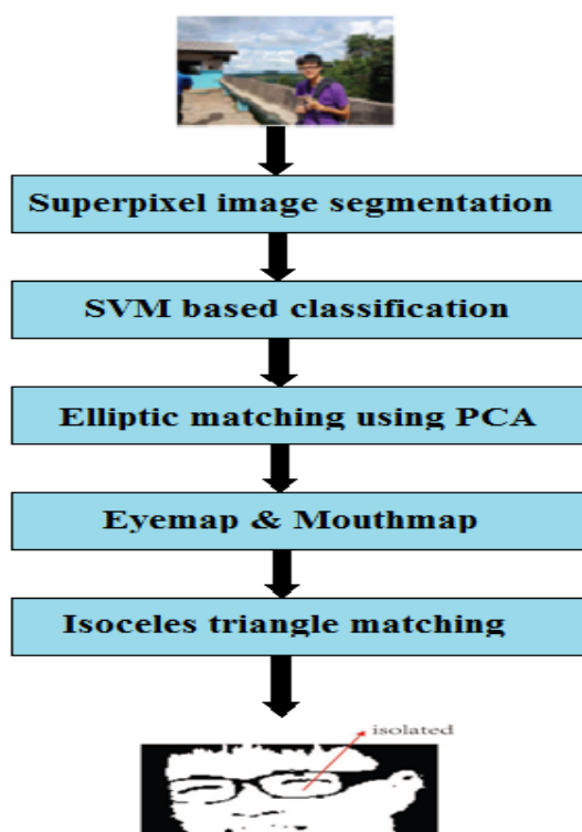
Fig.5. Superpixel based face detection algorithm
