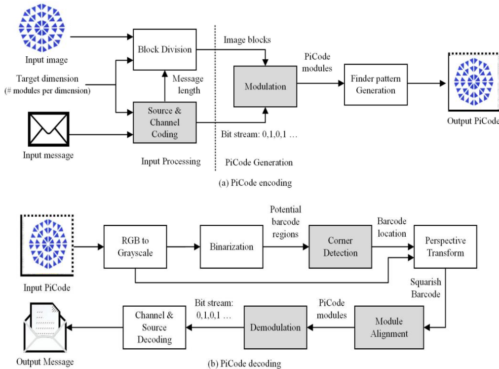
Fig.2.Block diagram of picode encoding and decoding
