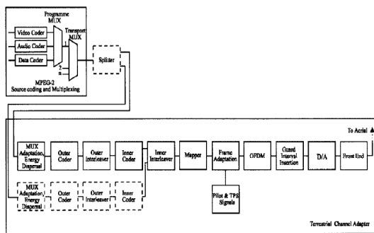
Figure 1.1: DVB-T transmitter [1]
