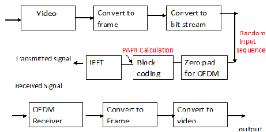
BLOCK DIAGRAM
