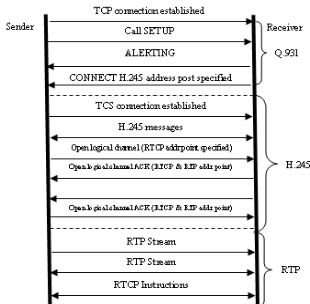
Fig. 3 Call Setup Process in H.323 [20]
