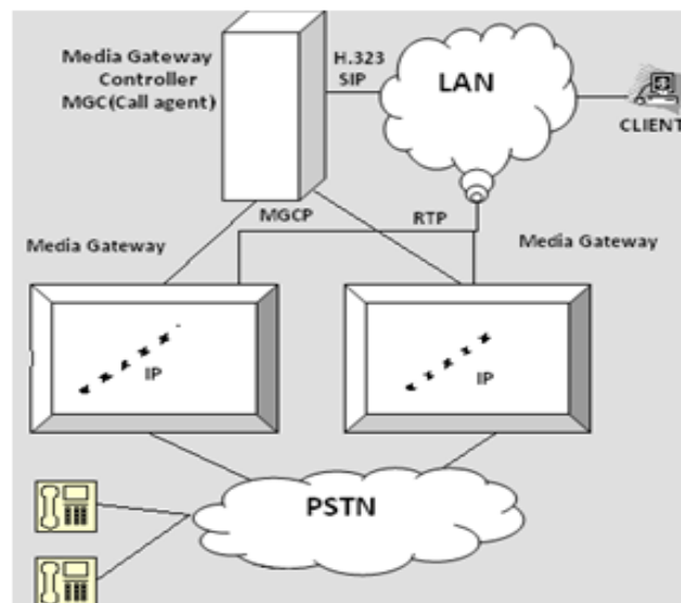
Fig. 6 MGCP Architecture [19]
