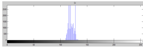
Fig.4.Histogram of Cr
