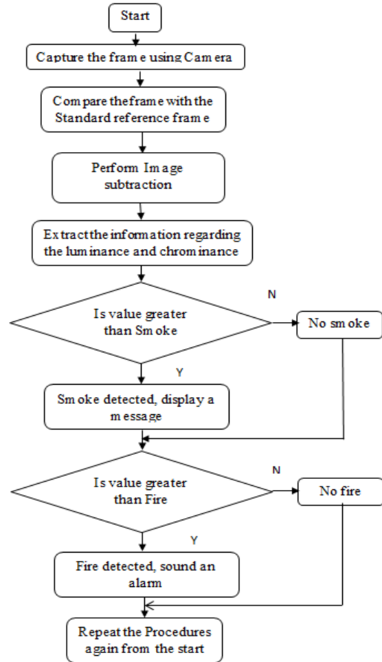
Fig. 1. Flowchart
