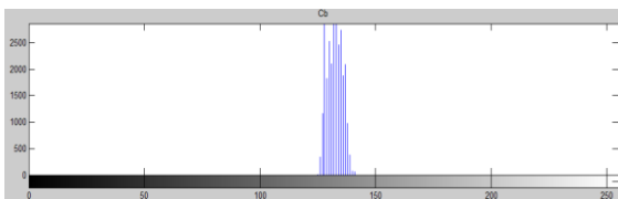
Fig.3.Histogram of Cb
