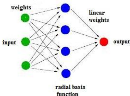
Fig2: Radial basis functions
