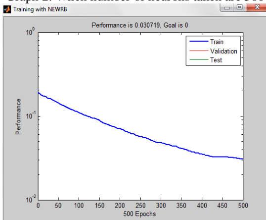
Graph 2: When number of neurons taken are 500
