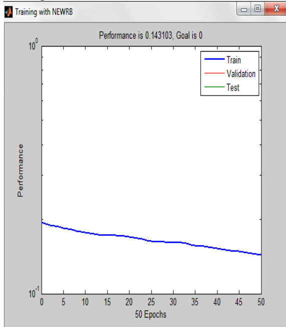
Graph1: when number of neurons taken are 50
