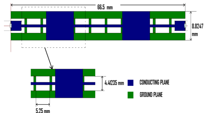
Figure 3: Dimensions of Stepped Impedance, L-C Ladder Type LPF (n=5) with PBG
