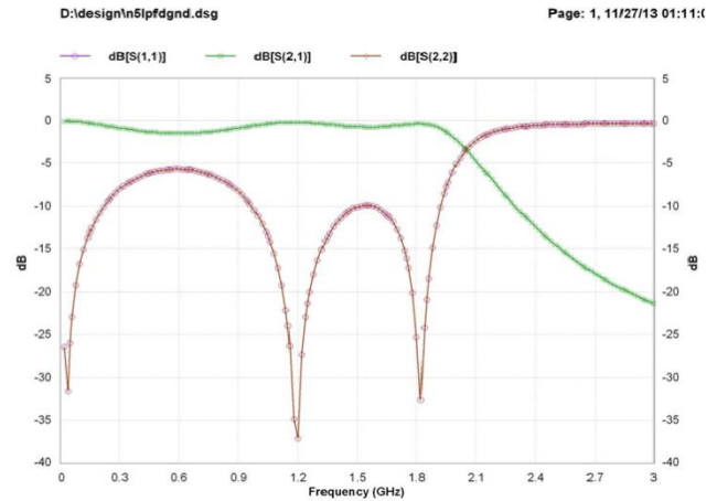
Figure 5: Simulated performance of stepped impedance, L-C ladder type with rectangular photonic band gap (PBG) LPF
