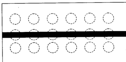
Fig.1 Microstrip with etched periodic pattern in ground plane
