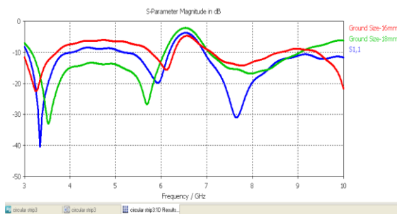
Figure 6: Effect of ground size variation on the antenna performance
