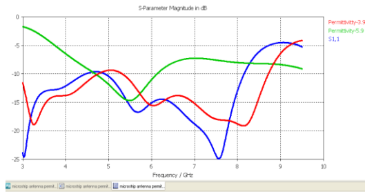
Figure 5 – Effect of substrate permittivity ( \epsilon_r ) on antenna performance characteristics
