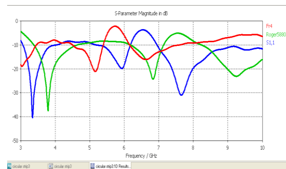
Figure 4: Effect of substrate material on the antenna performance
