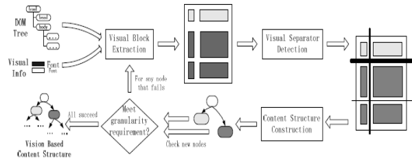
Fig.6. Flow of vision based page segmentation algorithm
