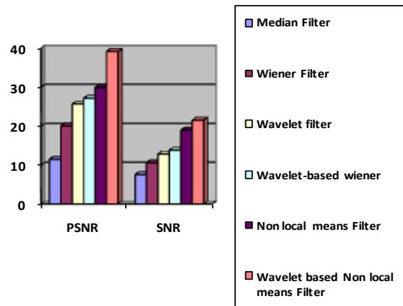
Fig 2: Analysis of PSNR and SNR values of various filter by adding additive white Gaussian noise of variance 10 and 20 .
