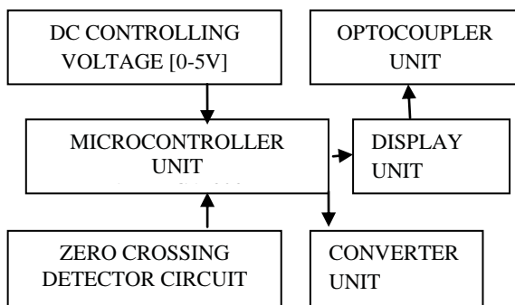
Fig. 1: Block diagram for controlling output power of converter
