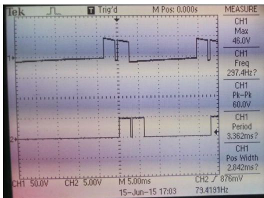
Fig.6: Train of pulses for triggering of SCR
