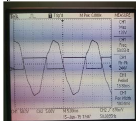
FIG 4 ZCD output
