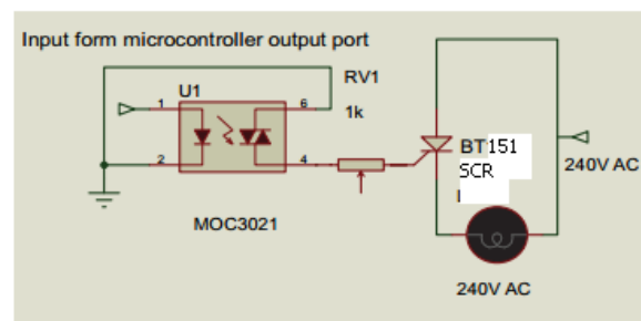
FIG 5 Optical isolation between control and load circuit.
