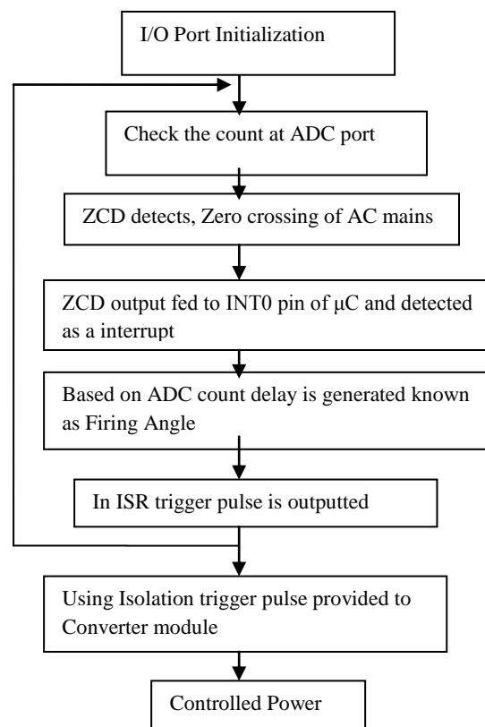
Fig. 3: Flowchart of digital triggering module
