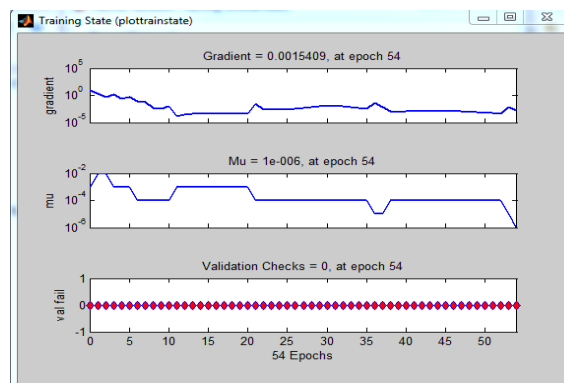
Fig 4: Training state plot of ANN with periodogram
