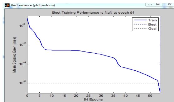
Fig 3: Performance plot of ANN with periodogram
