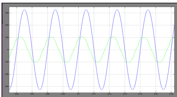
Fig. 7 Terminal voltages and source currents using the proposed method. Phase-a
