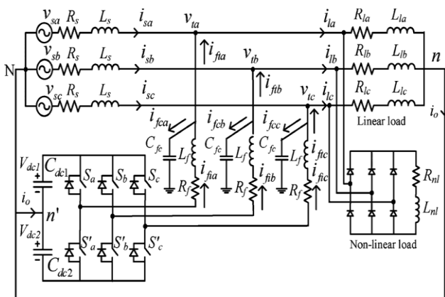
Fig. 1. Circuit diagram of the DSTATCOM-compensated distribution system.
