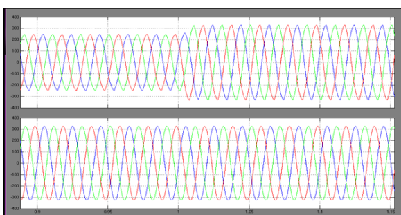
Fig. 11. (b) Source voltages during sag to normal.
