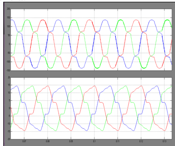
Fig. 4. Before compensation. (a) Terminal voltages. (b) Source currents.
