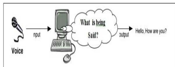
Figure 1: Speech Recognition
