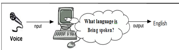
Figure 3: Language Identification
