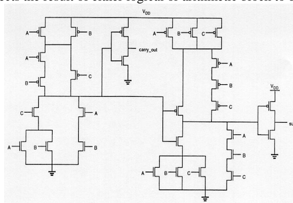
Figure 2: AdderDesign Block Diagram for Transistor Level
