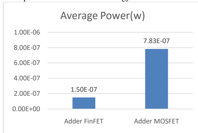
Figure 4: Adder Average Power for MOSFET and FinFET
