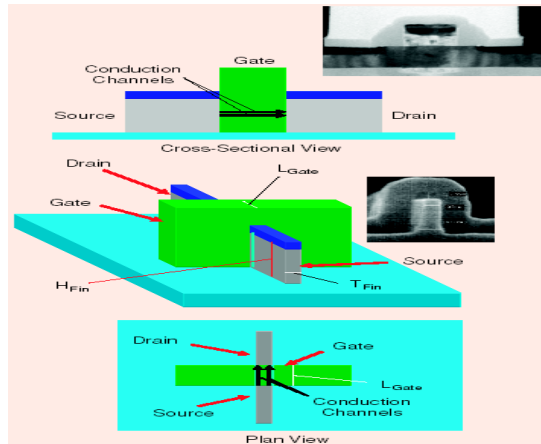
Figure 1 FinFET structure
