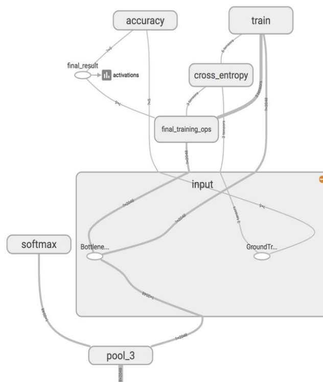
Figure 2. MobileNet model
