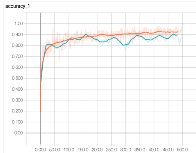
Figure 5. Accuracy with respect to training and validation
