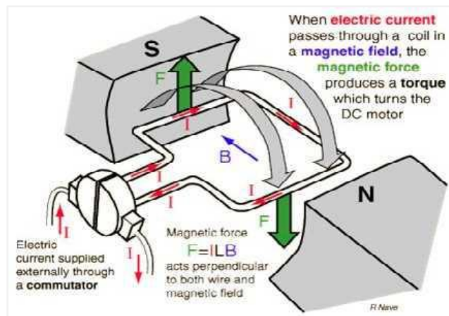
Fig6.Working of DC motor
