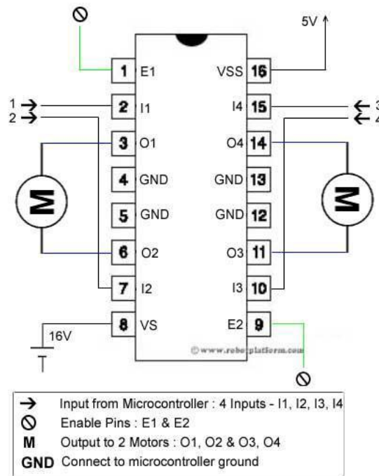
Fig7.Motor driver (L293D)
