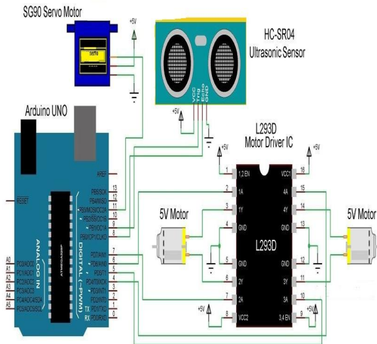
Fig8. Circuit diagram
