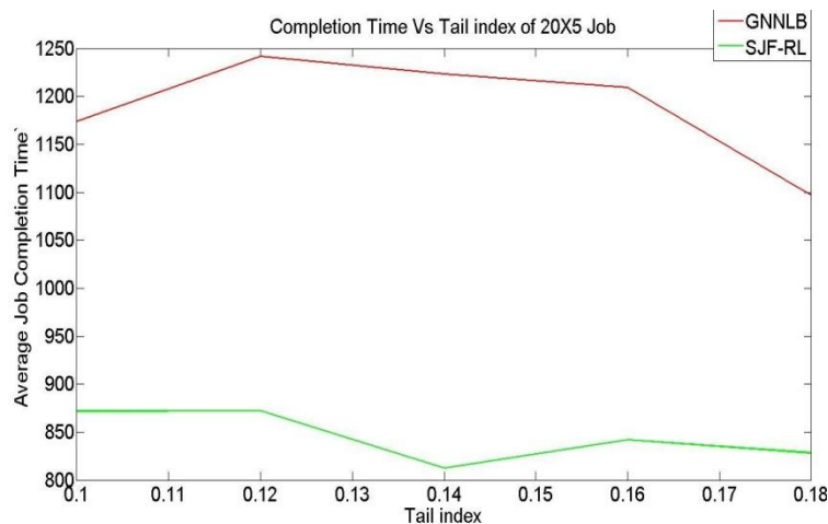
Fig. 3 Comparison of GNNLB and SJF-RL on the basis of arrival time tail index.
