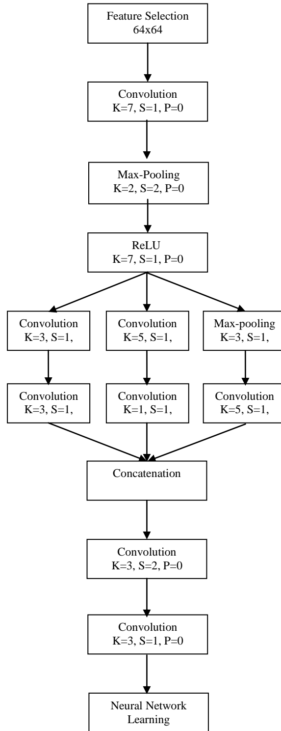
Fig. 2 Represent Block Diagram of GNNLB.
