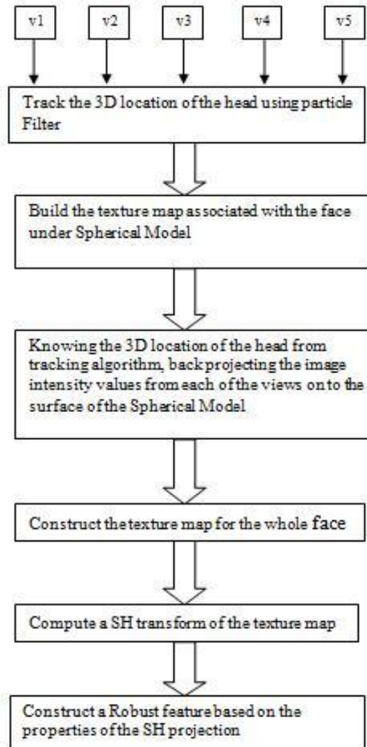
Fig 1: Flow diagram of Multi-view Face Recognition Algorithm
