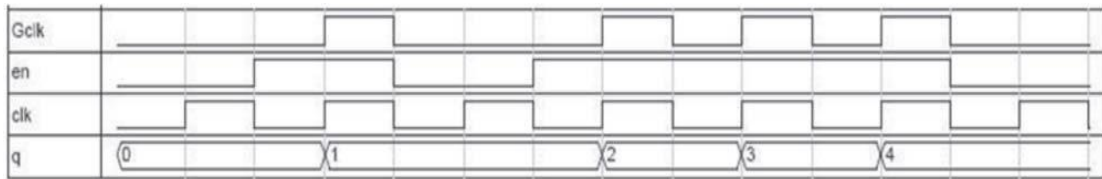
Figure (D): Right Output when counters positive edge triggered.
