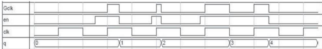
Figure (E): Hazards Problem when AND clock gating Circuitry used.
