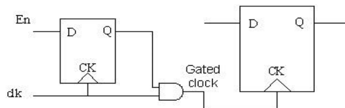
Figure : Clock Gating.
