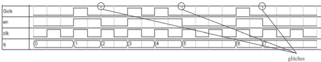
Figure (C): Wrong Output due to Glitch, when counters Positive edge triggered.
