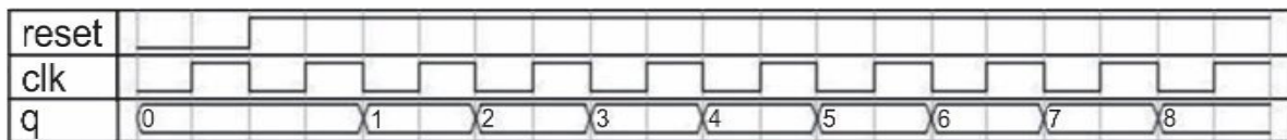
Figure (B): Normal output of the counter without Clock Gating.
