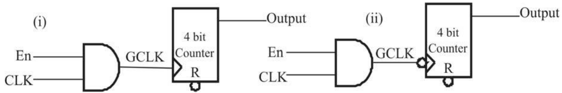
Figure (A): Clock gating using AND gate Circuit.
