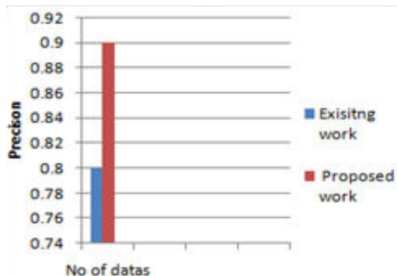
Fig. 1 Precision comparison
