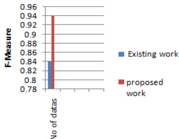
Fig. 3 F-Measure comparison
