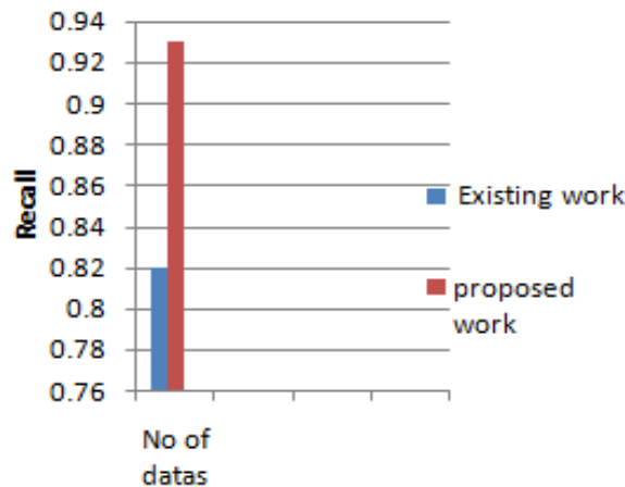
Fig. 2 Recall Comparison
