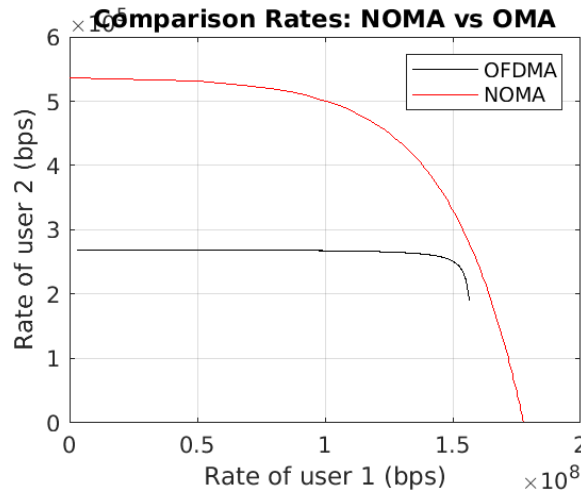
Figure 7 Rate pairs with OFDMA and NOMA for downlink PD-NOMA for Small urban areas
