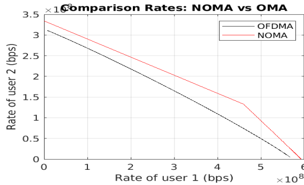
Figure 10 Rate pairs with OFDMA and NOMA for downlink PD-NOMA for Rural areas
