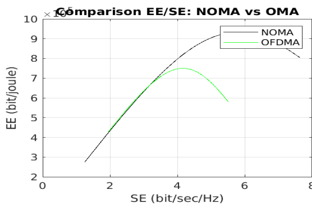
Figure 12 EE-SE trade-off curves for PD-NOMA OFDMA for Metropolitan urban areas
