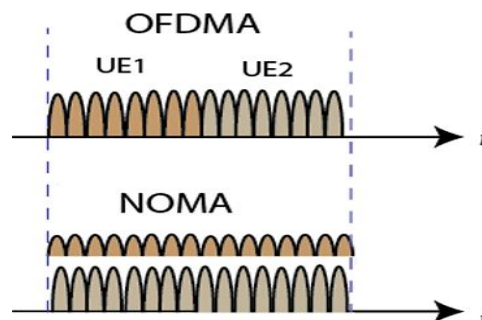
Figure 1 Spectrum sharing for OFDMA and NOMA for two users.
