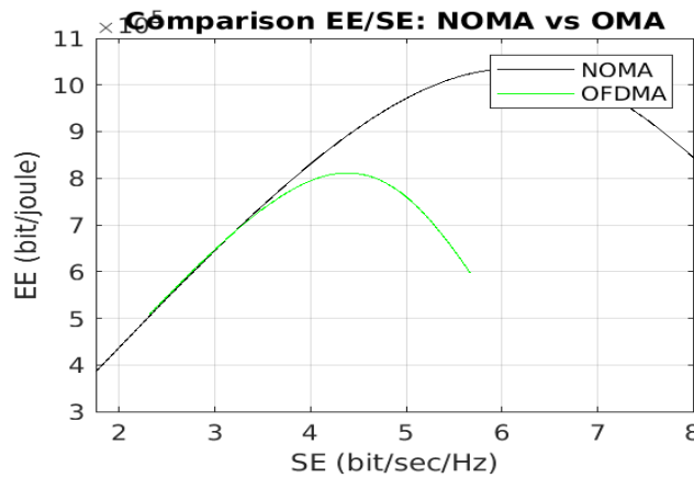
Figure 11 EE-SE trade-off curves for PD-NOMA OFDMA for Small urban areas
