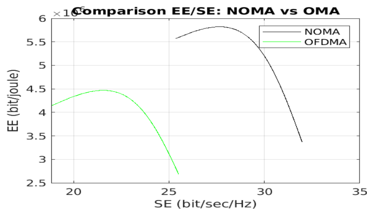
Figure 14 EE-SE trade-off curves for PD-NOMA OFDMA for Rural areas
