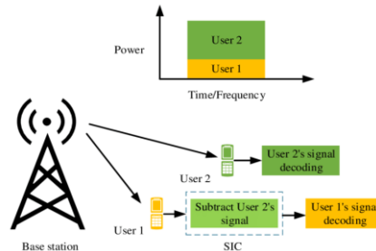
Figure 4 Downlink Transmission
