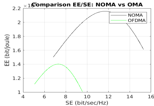
Figure 13 EE-SE trade-off curves for PD-NOMA OFDMA for Sub urban areas
