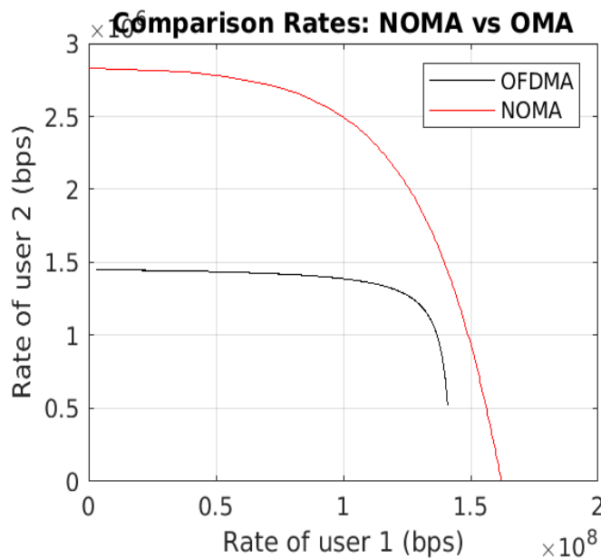
Figure 8 Rate pairs with OFDMA and NOMA for downlink PD-NOMA for Metropolitan urban areas
