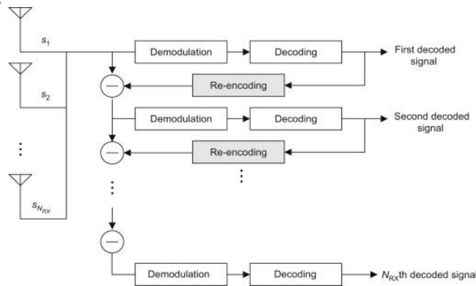
Figure 6 Successive interference cancellation
