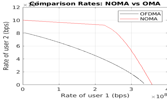
Figure 9 Rate pairs with OFDMA and NOMA for downlink PD-NOMA for Sub-urban areas
