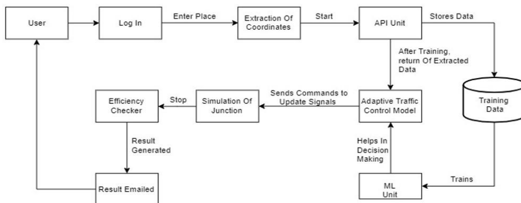
Fig 1. Architecture Diagram
