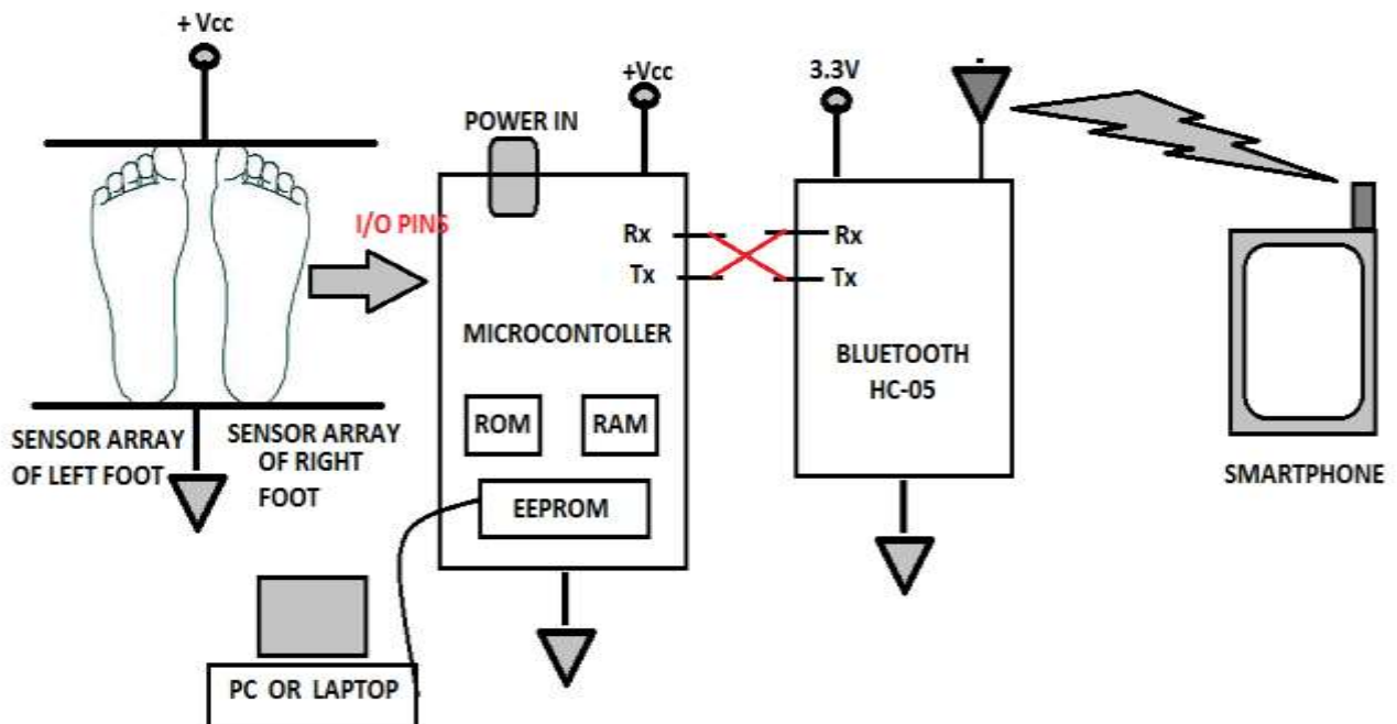
Figure 3 Block diagram
