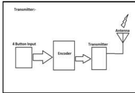
Fig. 2.2.1 Transmitter
