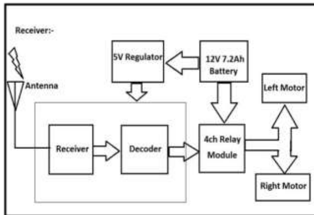
Fig.2.2.2 Receiver
