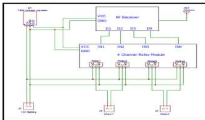
Fig.2.3.1 Relay kit
