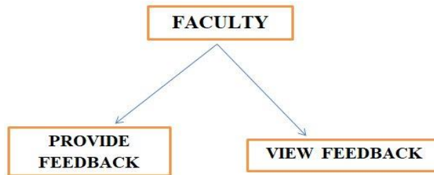
Fig. IV FACULTY MODULE
