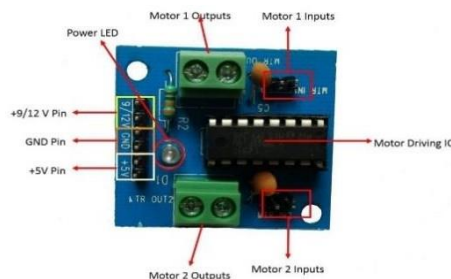
Figure 6 Motor Driver IC (L293D)
