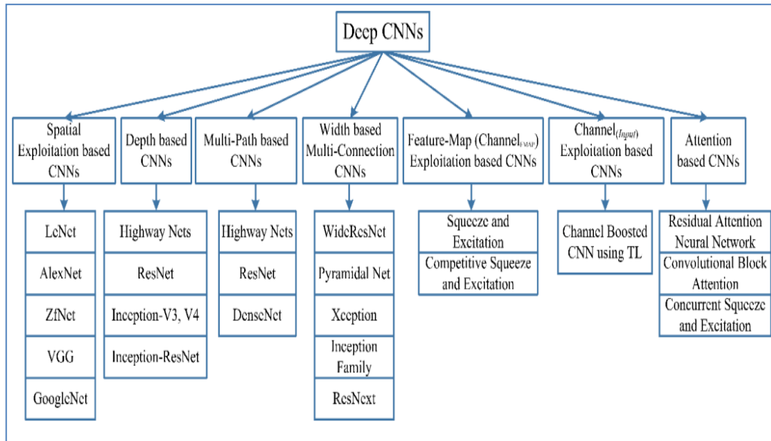
Figure 6 : Taxonomy of deep CNN architectures showing seven different categories [26]
