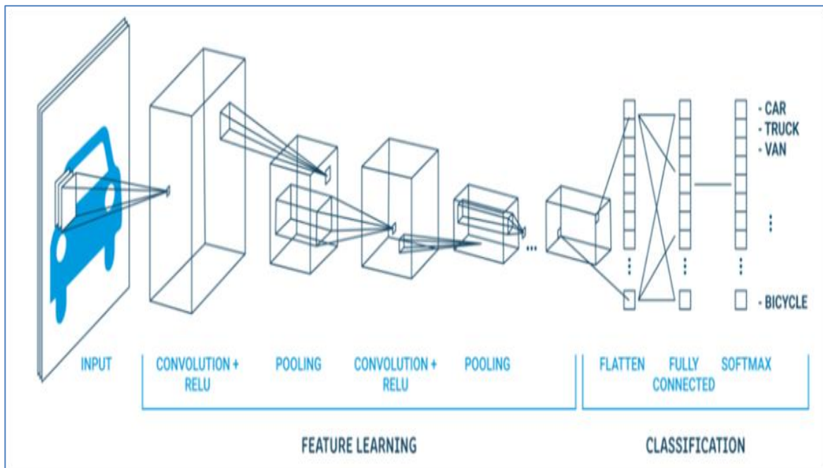
Figure 5: Deep Convolution Neural Network Architecture [24]
