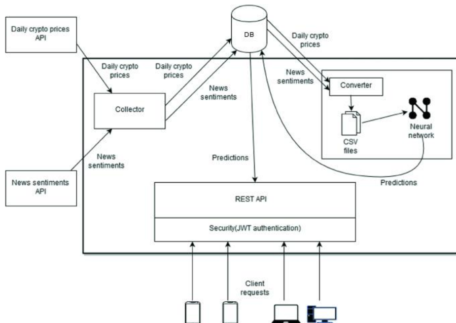
Fig 1: Cryptocurrency price prediction system
