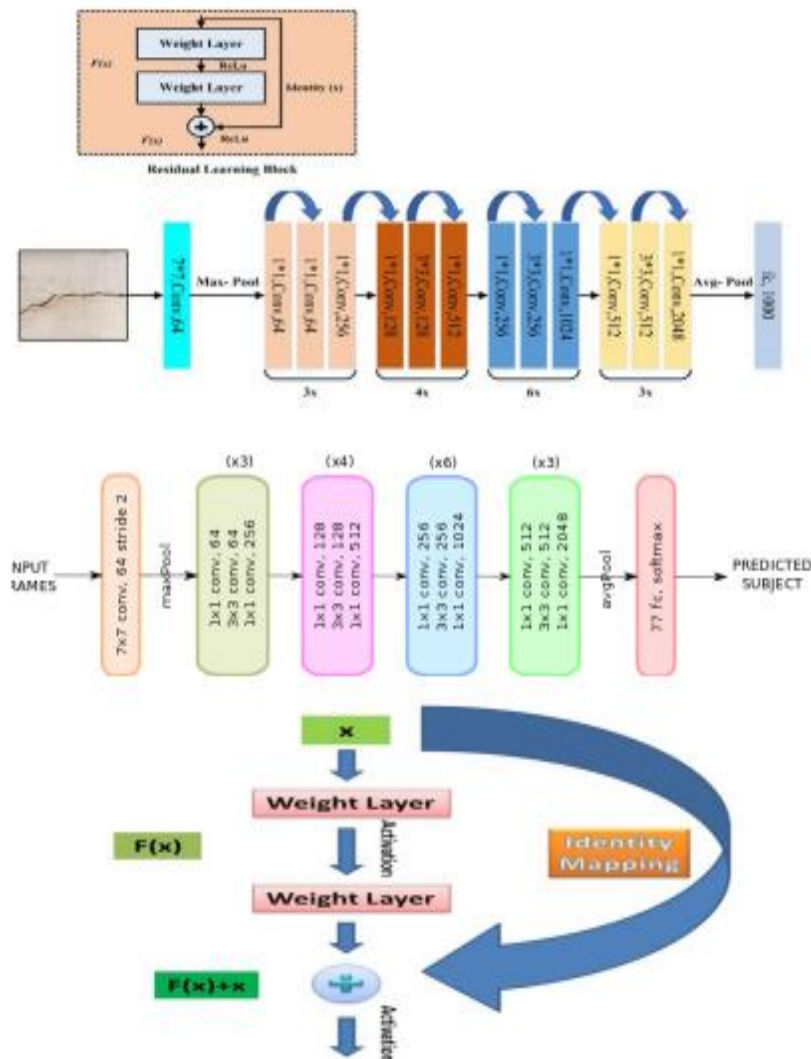
Fig 4: ResNet-50 neural network architecture
