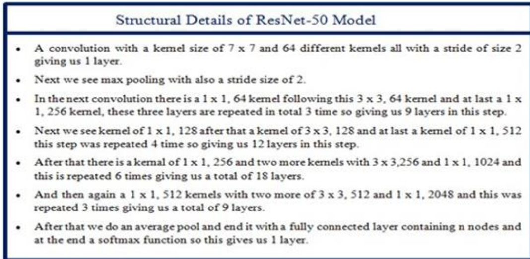
Fig 3: Internal structural details of the ResNet-50 architecture.
