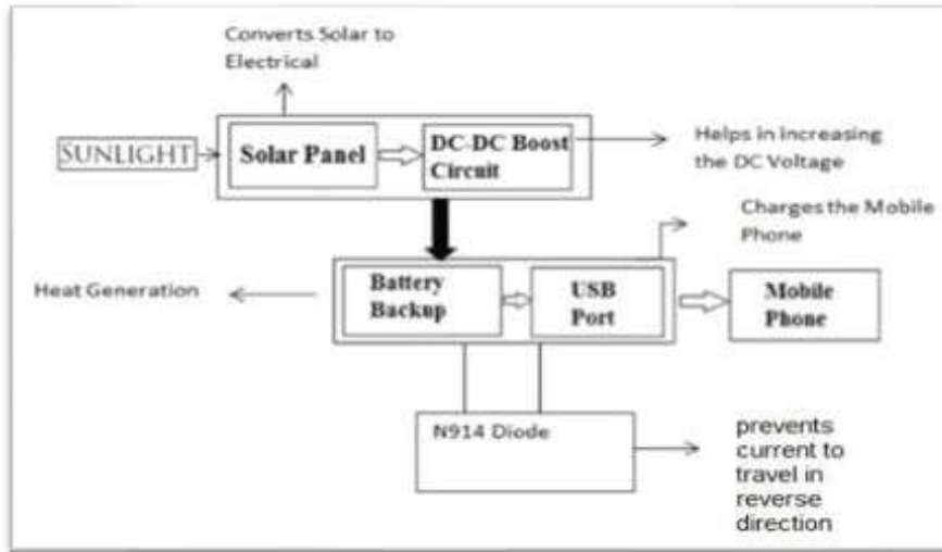
Fig.1: Block Diagram.
