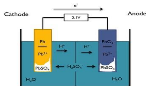
Figure. Chemical reaction in Lead acid battery
