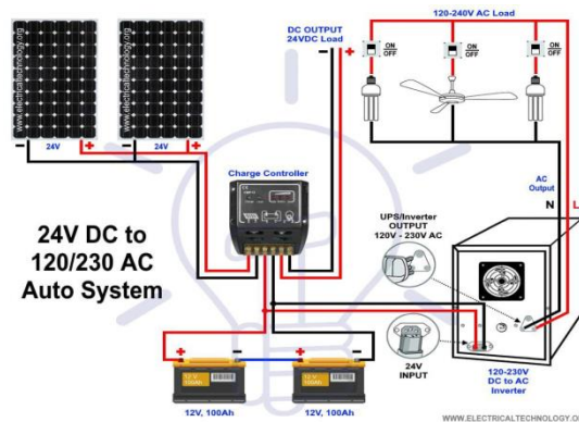
Figure: Connection diagram of Off-Grid PV system
